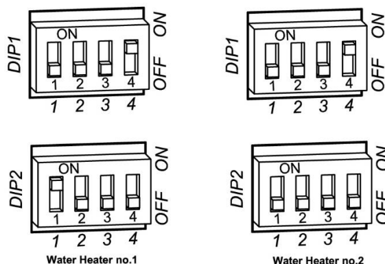
dip switch settings without temperature controller
