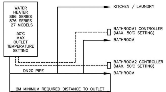
876 Series - Bathroom Controllers Only
