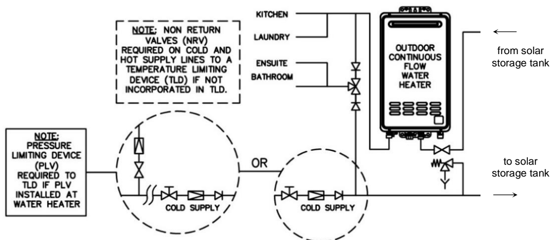
In-series Gas Booster as part of a Closed Circuit Solar Water Heater Installation Two Temperature Zones Using a Temperature Limiting Device
