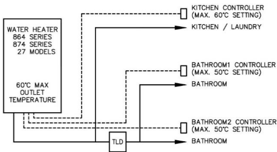
Note: NZ - Kitchen Controller max setting is 55°C 874 Series - Kitchen Controller Only
