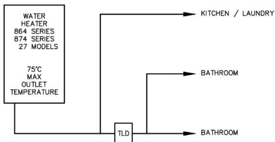
874 Series - Bathroom Controllers Only
