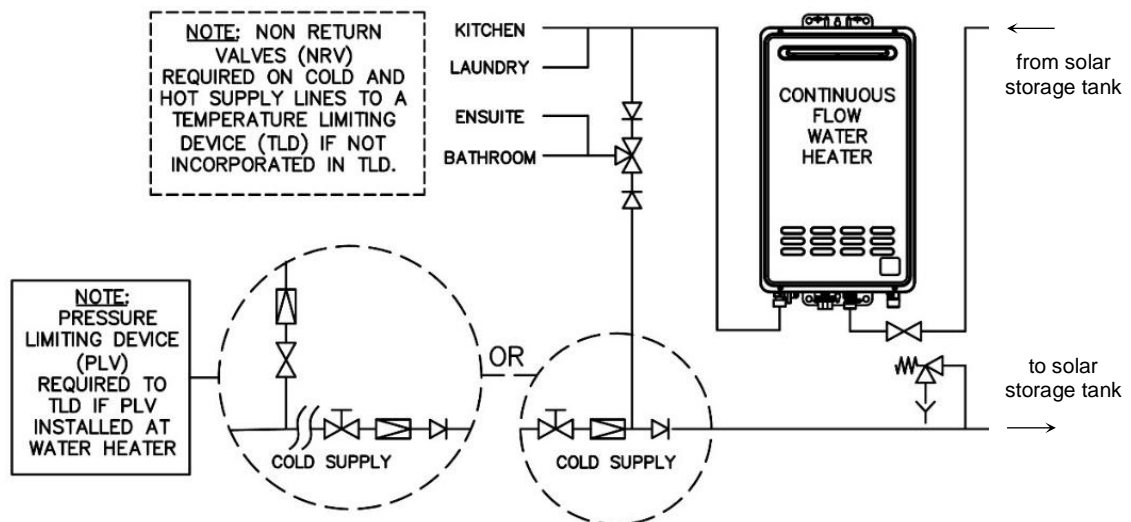
In-series Gas Booster as part of an Open Circuit Solar Water Heater Installation Two Temperature Zones Using a Temperature Limiting Device
