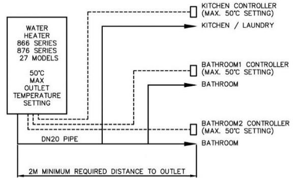
876 Series – Kitchen and Bathroom Controllers
